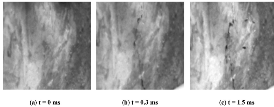
Fig. 14. Dynamic performance of the UHPFRC with hybrid fibres (HF + LSF) under the bullet (7.62 mm, velocity \approx 830 \text{ m/s} ) impact (rear surface, first shot).
