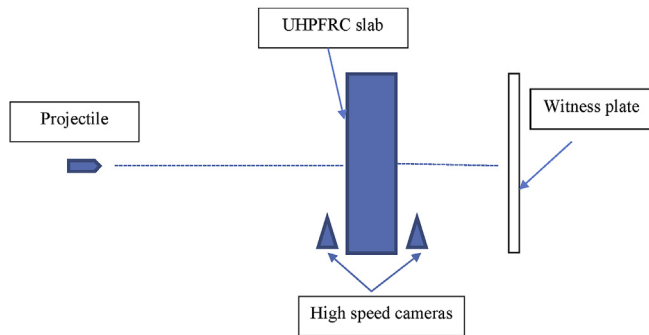
Fig. 6. Scheme of the projectile impact tests.
