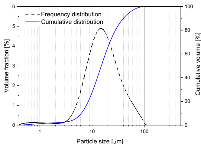
Fig. 1. The particle size distribution of BOF slag.
