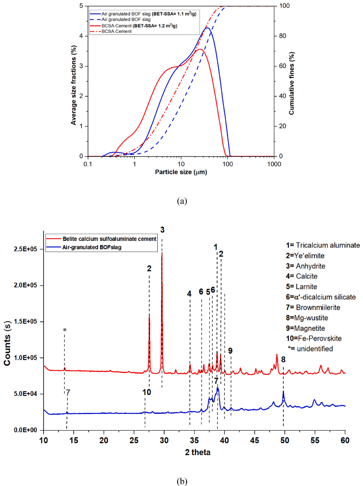
Fig. 1. a) The PSD (particle size distribution) of the raw material. In the inset, specific surface area (SSA) is obtained via the BET method. b) X-ray diffraction pattern of BCSA and air granulated BOF slag with labeled peaks.
