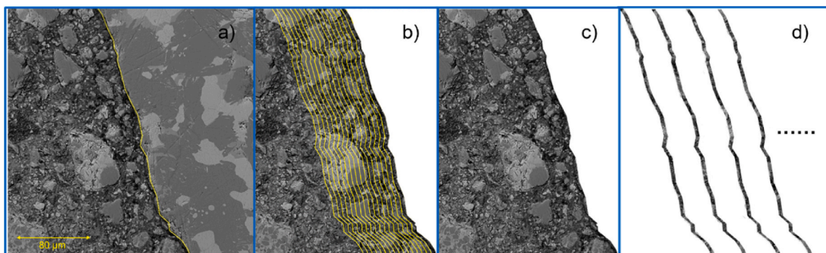
Fig. 3. The schematic diagram for the processing of a typical BSE image.
