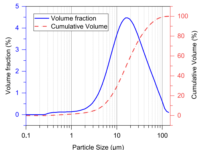
Fig. 1. Particle size distribution of milled BOF slag.
