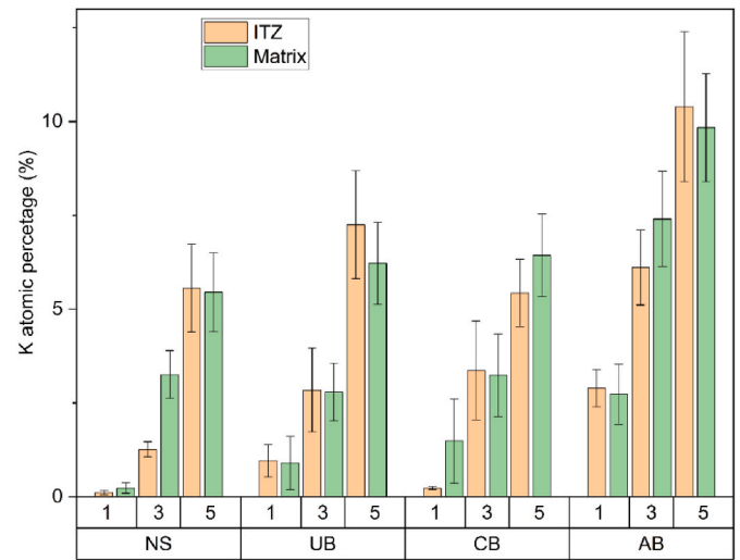
Fig. 17. Comparison of K atomic concentration within ITZ and matrix.
